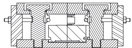
Section Z-Z
